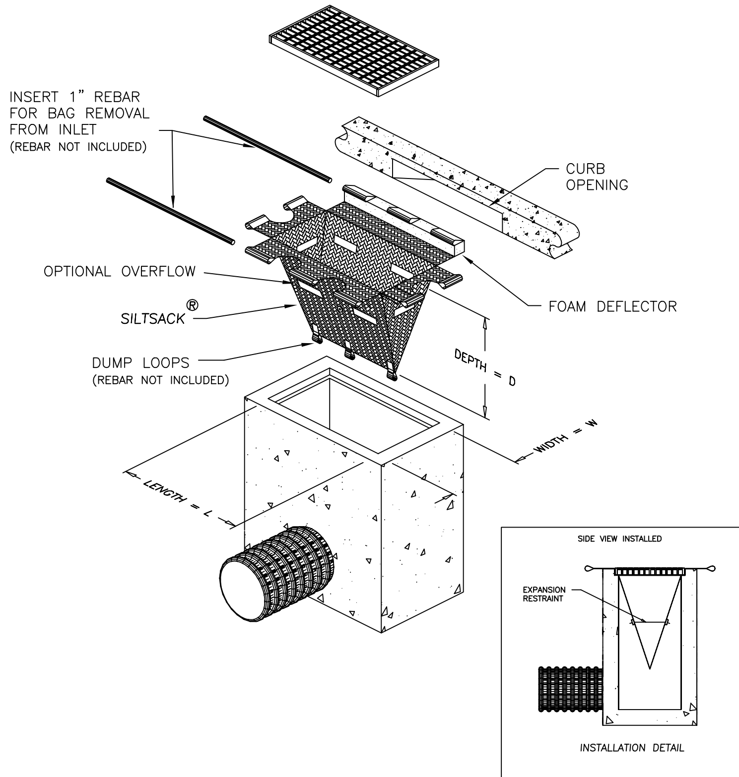
DETAIL OF INLET SEDIMENT CONTROL DEVICE TYPE B – WITH FOAM DEFLECTOR
